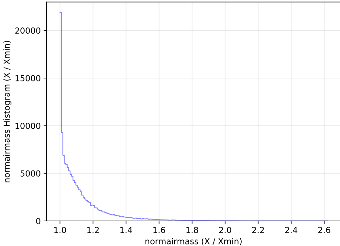
internal_u_expt27_nscale1.1v3.4_10yrs All sky u band: normairmass Histogram
