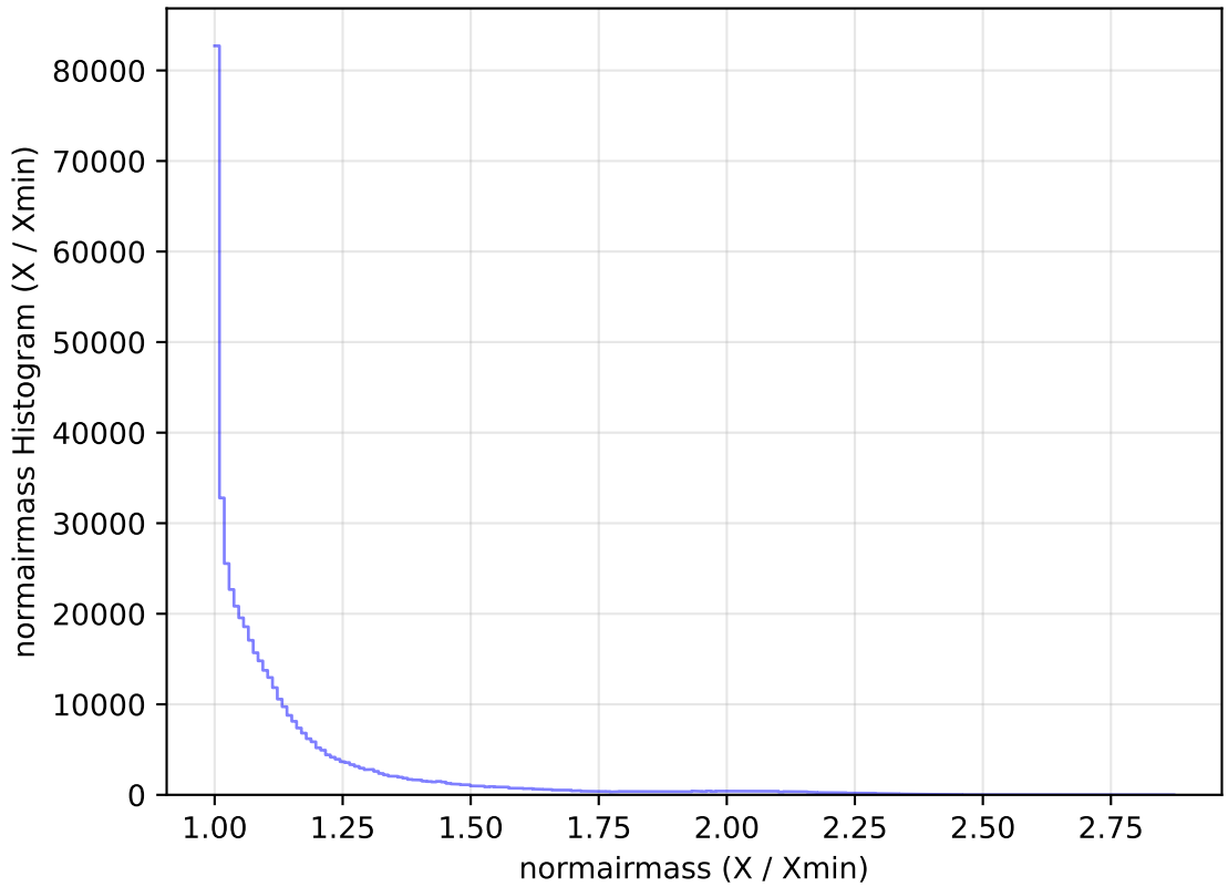
internal_u_expt27_nscale1.1v3.4_10yrs All sky r band: normairmass Histogram
