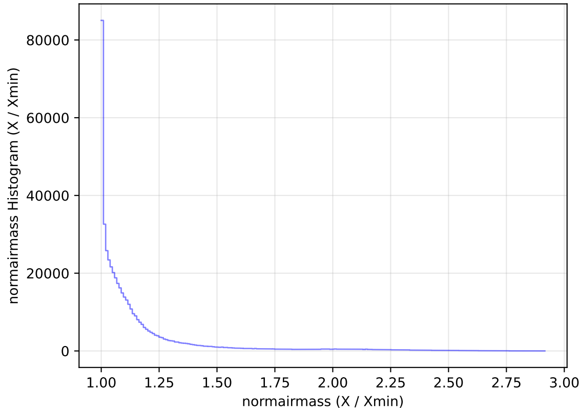
internal_u_expt27_nscale1.1v3.4_10yrs All sky i band: normairmass Histogram
