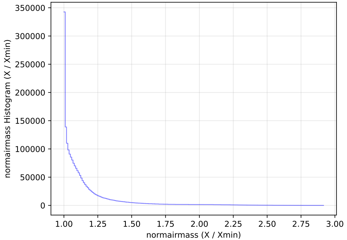
internal_u_expt27_nscale1.1v3.4_10yrs All sky all bands: normairmass Histogram
