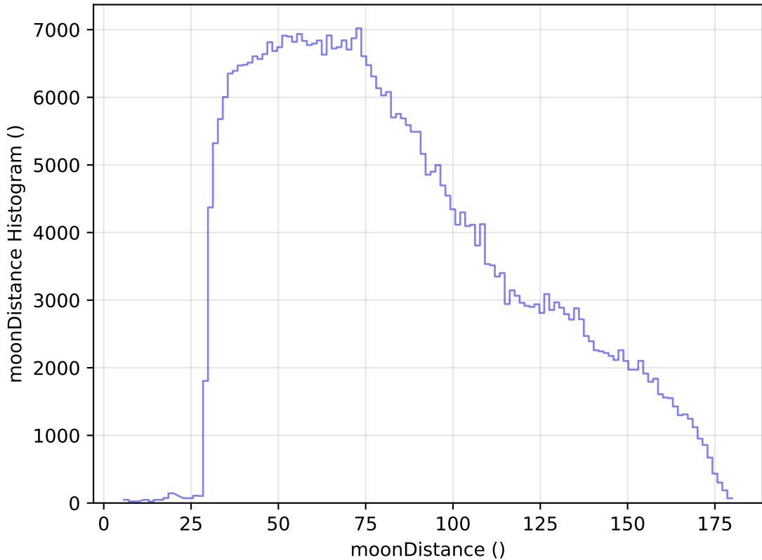
internal_u_expt27_nscale1.1v3.4_10yrs WFD z band: moonDistance Histogram
