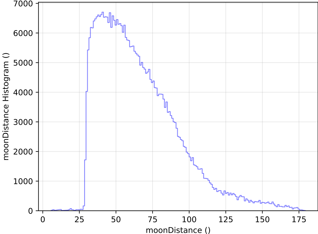
internal_u_expt27_nscale1.1v3.4_10yrs WFD y band: moonDistance Histogram
