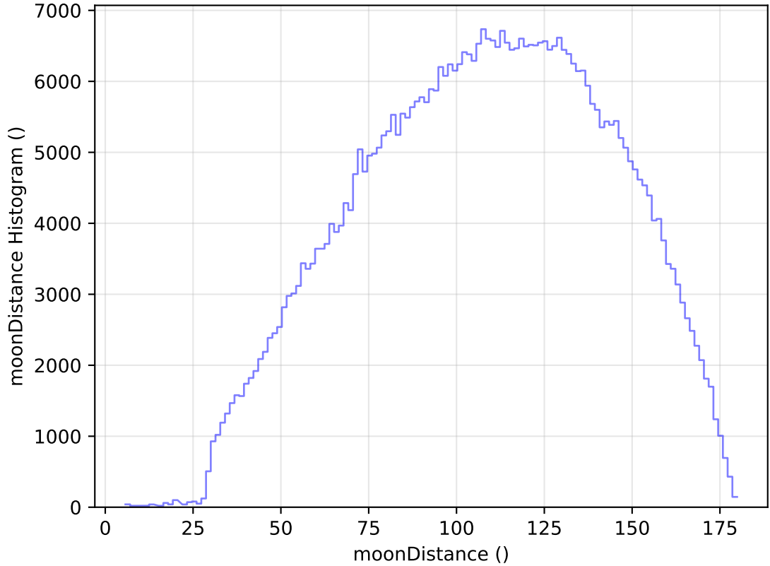
internal_u_expt27_nscale1.1v3.4_10yrs WFD r band: moonDistance Histogram
