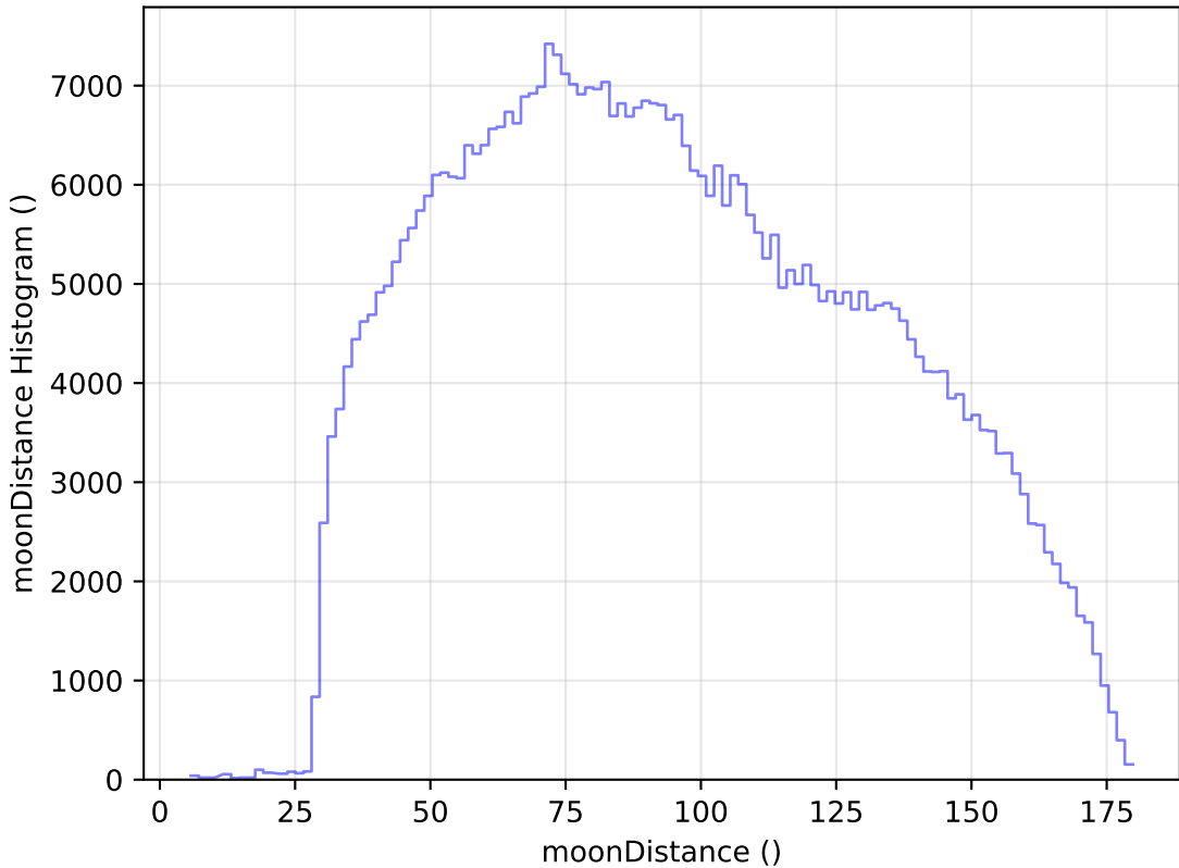
internal_u_expt27_nscale1.1v3.4_10yrs WFD i band: moonDistance Histogram
