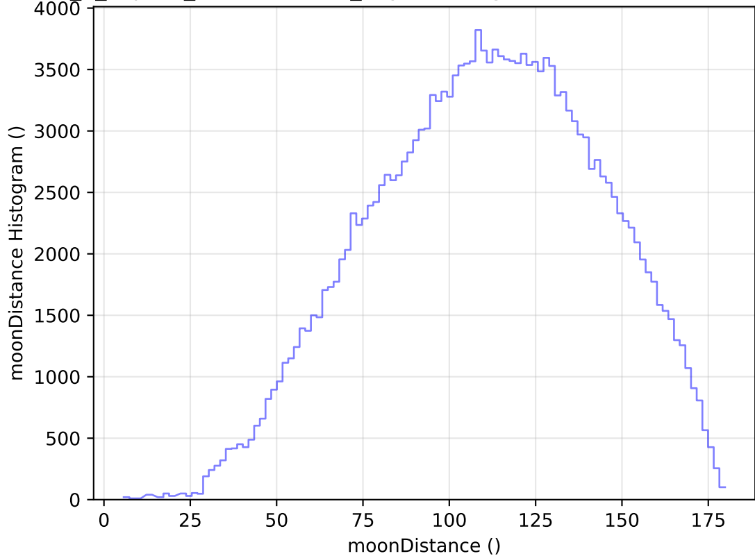
internal_u_expt27_nscale1.1v3.4_10yrs WFD g band: moonDistance Histogram
