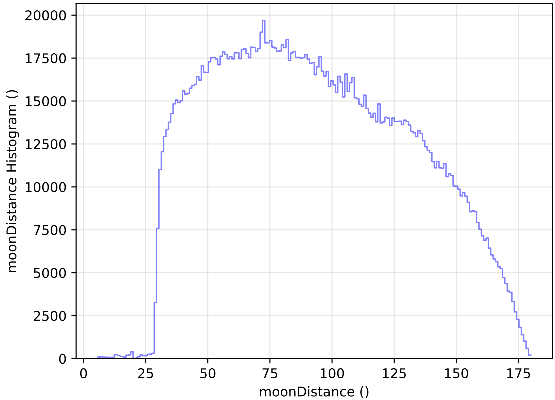
internal_u_expt27_nscale1.1v3.4_10yrs WFD all bands: moonDistance Histogram
