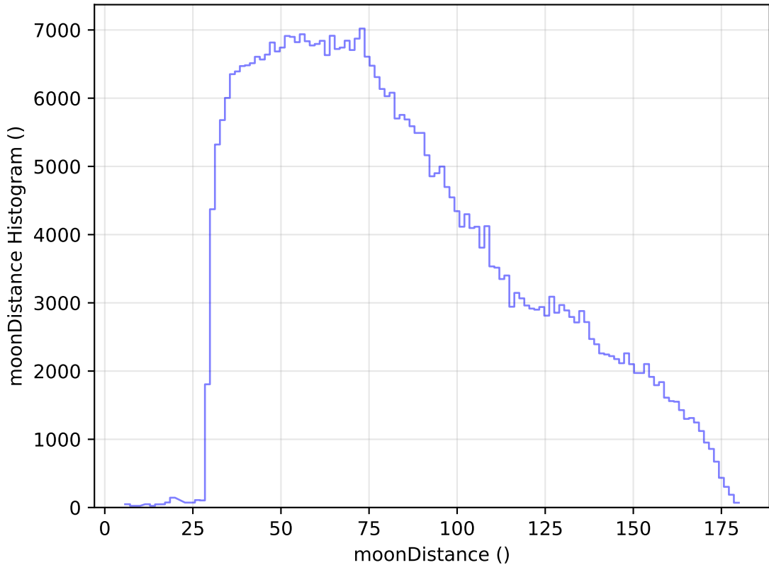
internal_u_expt27_nscale1.1v3.4_10yrs All sky z band: moonDistance Histogram
