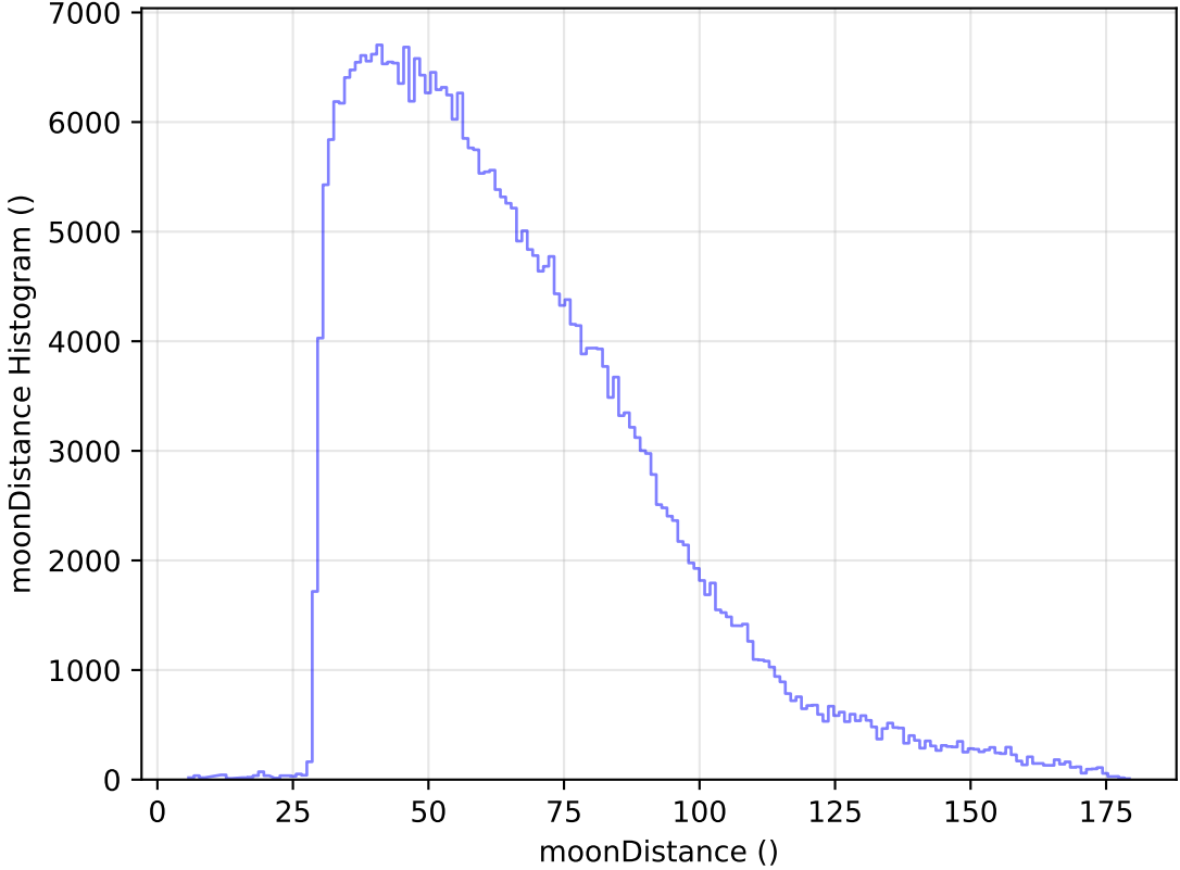
internal_u_expt27_nscale1.1v3.4_10yrs All sky y band: moonDistance Histogram
