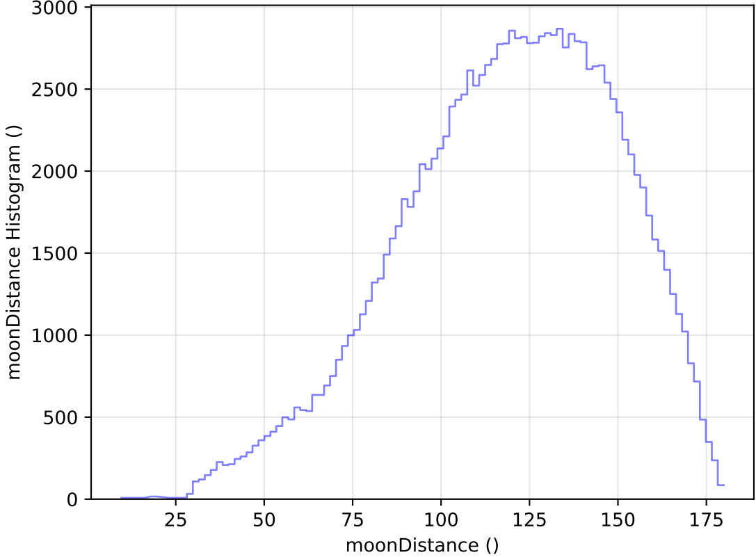
internal_u_expt27_nscale1.1v3.4_10yrs All sky u band: moonDistance Histogram
