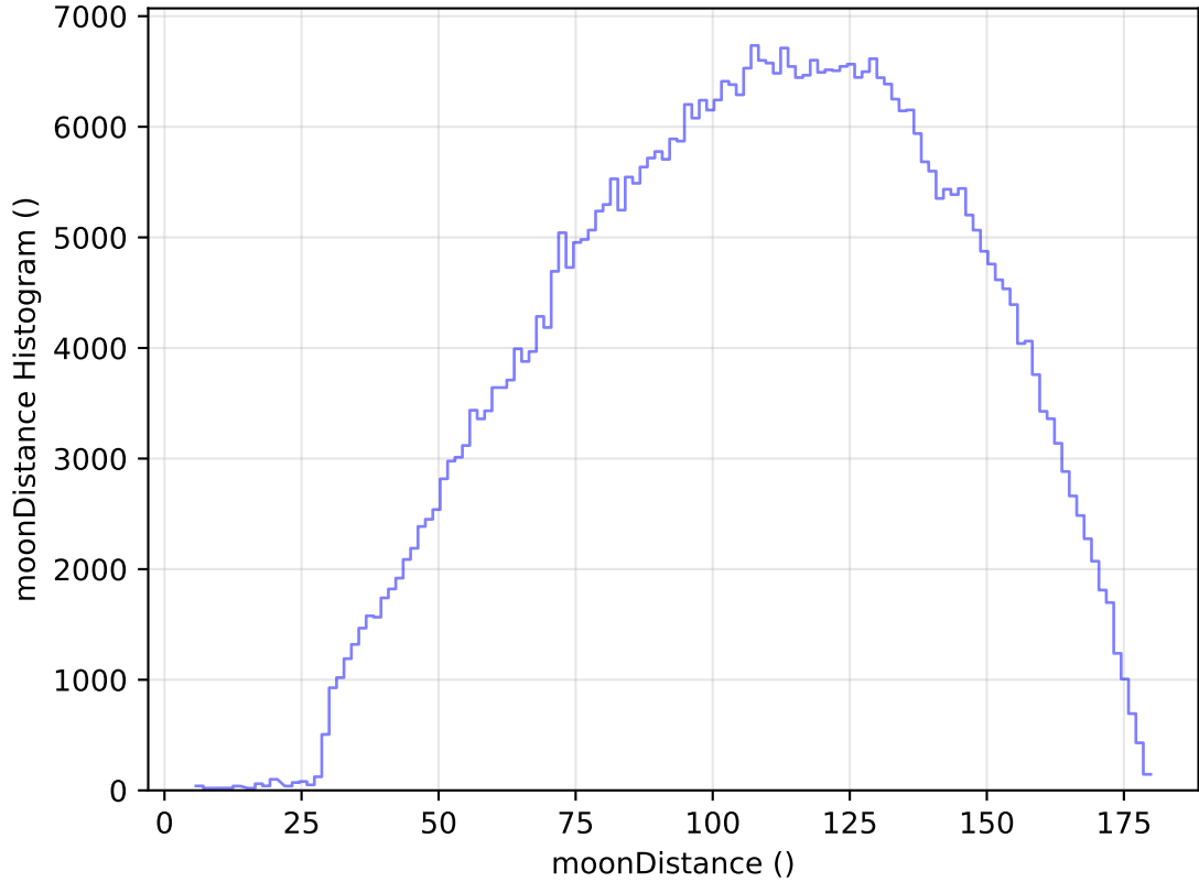
internal_u_expt27_nscale1.1v3.4_10yrs All sky r band: moonDistance Histogram
