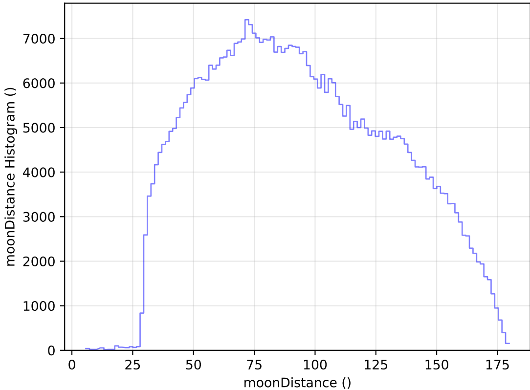
internal_u_expt27_nscale1.1v3.4_10yrs All sky i band: moonDistance Histogram
