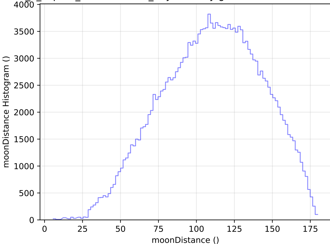
internal_u_expt27_nscale1.1v3.4_10yrs All sky g band: moonDistance Histogram
