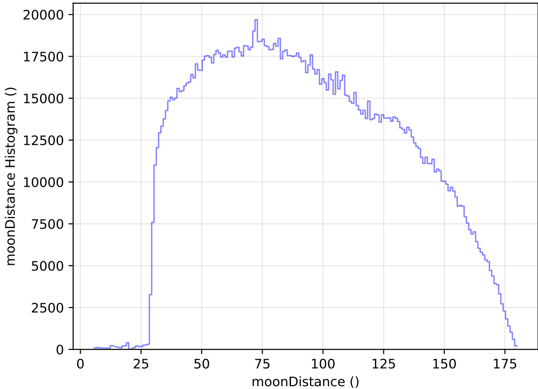
internal_u_expt27_nscale1.1v3.4_10yrs All sky all bands: moonDistance Histogram
