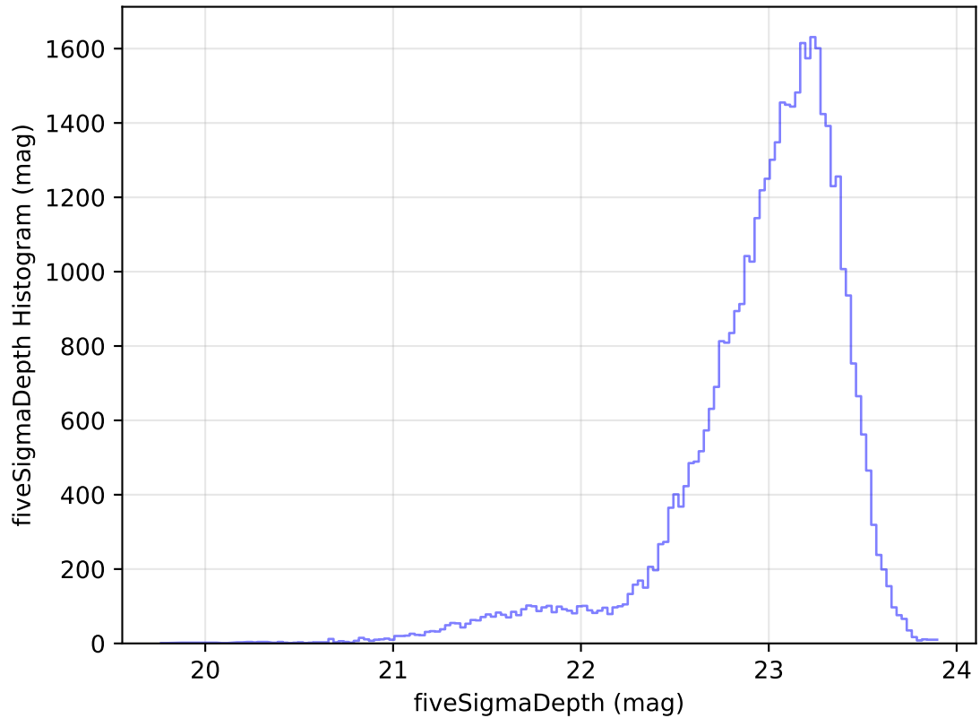
internal_u_expt27_nscale1.1v3.4_10yrs Yr 1 z band: fiveSigmaDepth Histogram
