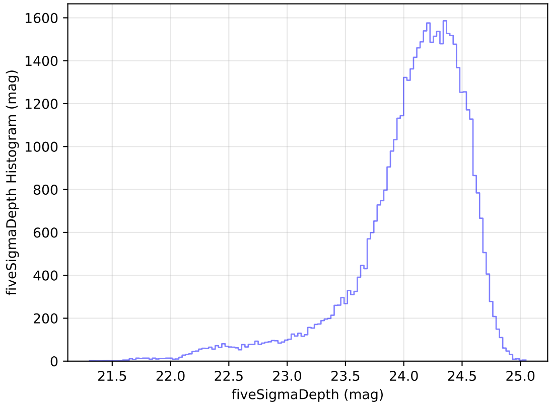
internal_u_expt27_nscale1.1v3.4_10yrs Yr 1 r band: fiveSigmaDepth Histogram
