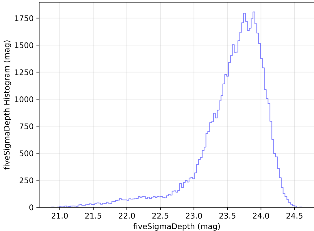
internal_u_expt27_nscale1.1v3.4_10yrs Yr 1 i band: fiveSigmaDepth Histogram
