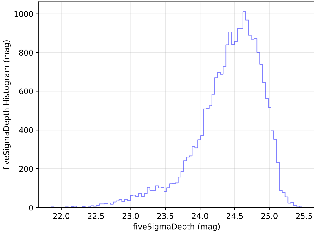
internal_u_expt27_nscale1.1v3.4_10yrs Yr 1 g band: fiveSigmaDepth Histogram
