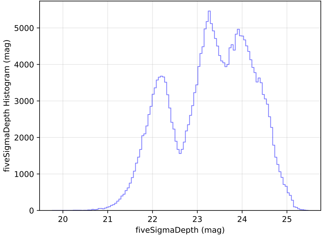
internal_u_expt27_nscale1.1v3.4_10yrs Yr 1 all bands: fiveSigmaDepth Histogram
