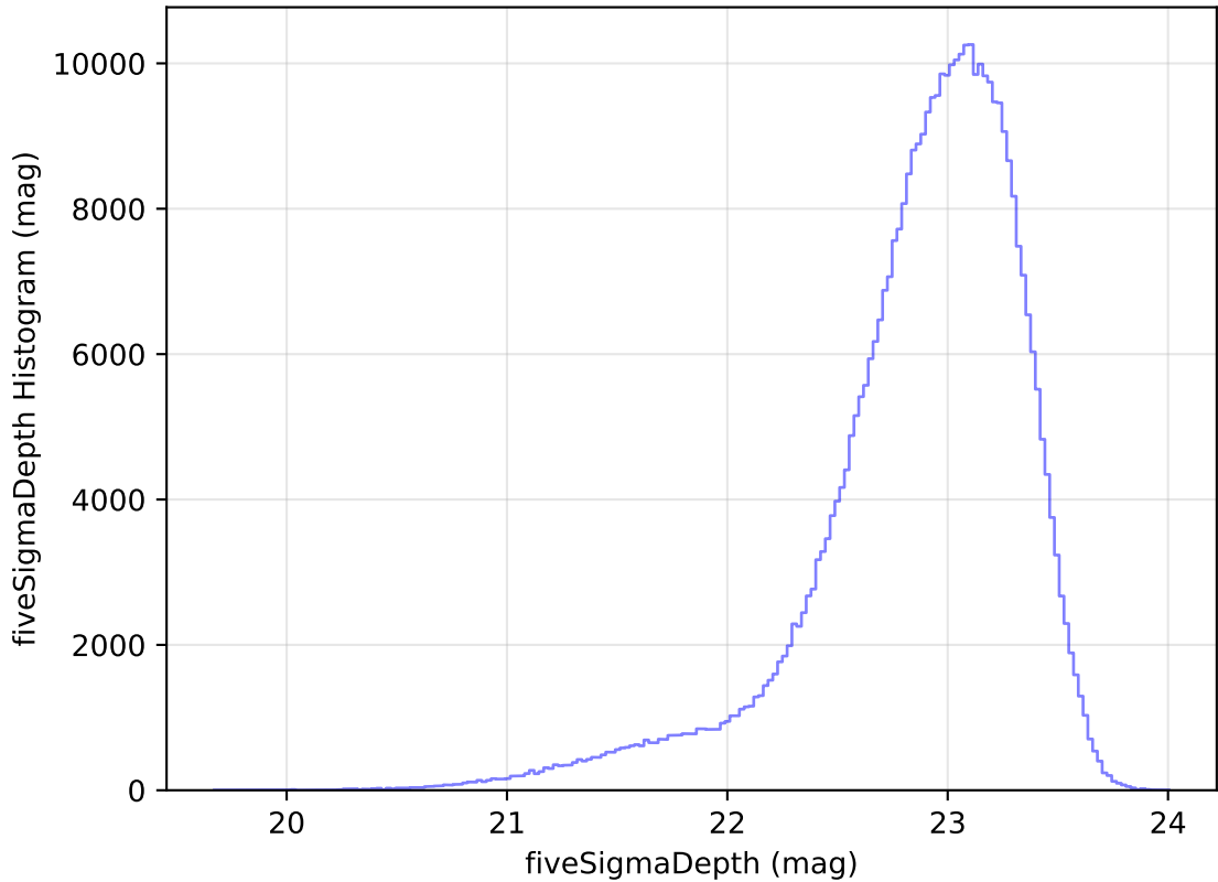
internal_u_expt27_nscale1.1v3.4_10yrs WFD z band: fiveSigmaDepth Histogram
