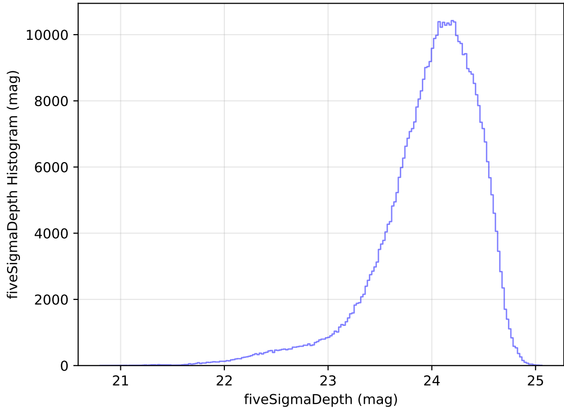
internal_u_expt27_nscale1.1v3.4_10yrs WFD r band: fiveSigmaDepth Histogram
