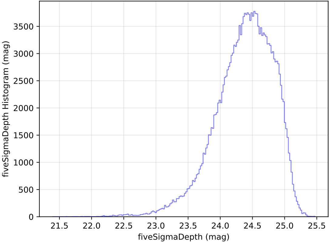
internal_u_expt27_nscale1.1v3.4_10yrs WFD g band: fiveSigmaDepth Histogram
