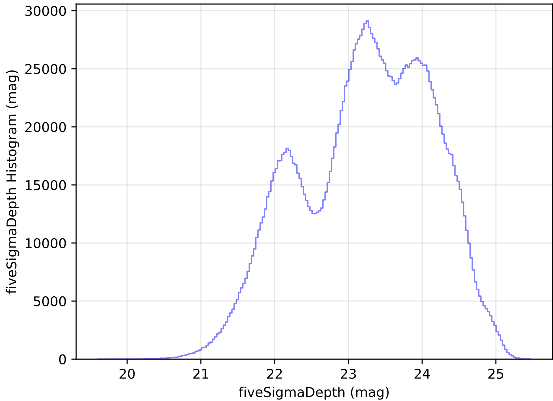
internal_u_expt27_nscale1.1v3.4_10yrs WFD all bands: fiveSigmaDepth Histogram
