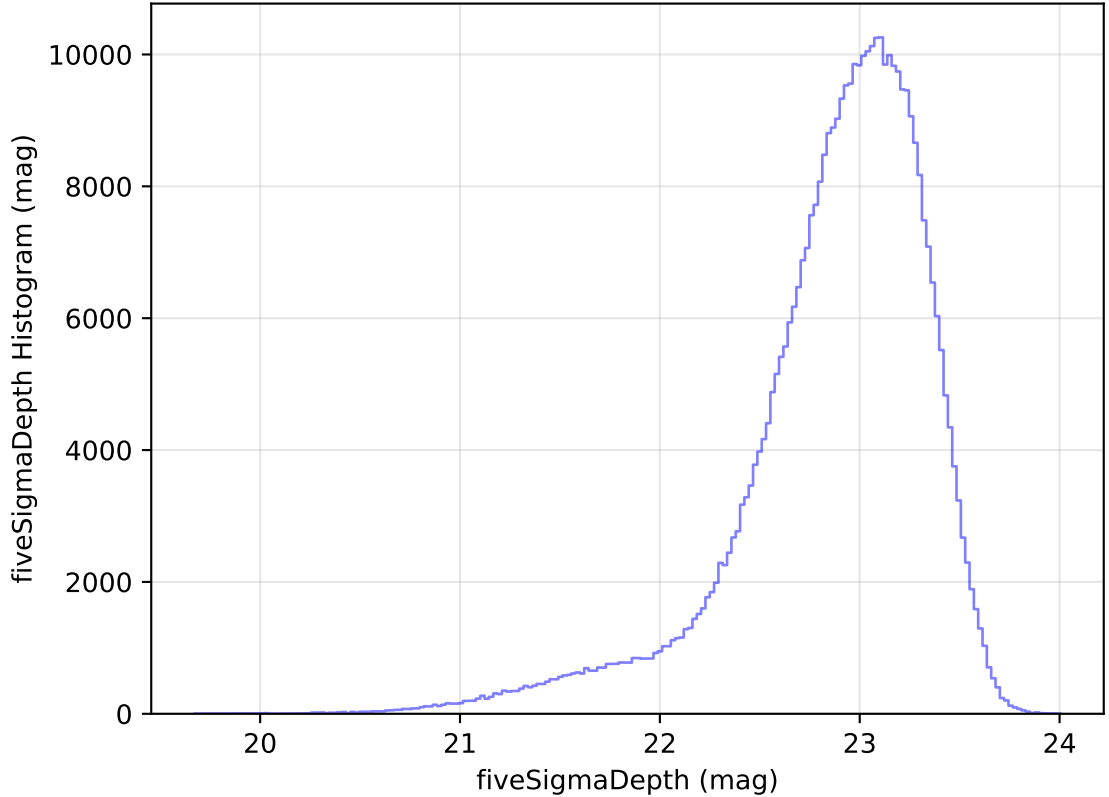
internal_u_expt27_nscale1.1v3.4_10yrs All sky z band: fiveSigmaDepth Histogram
