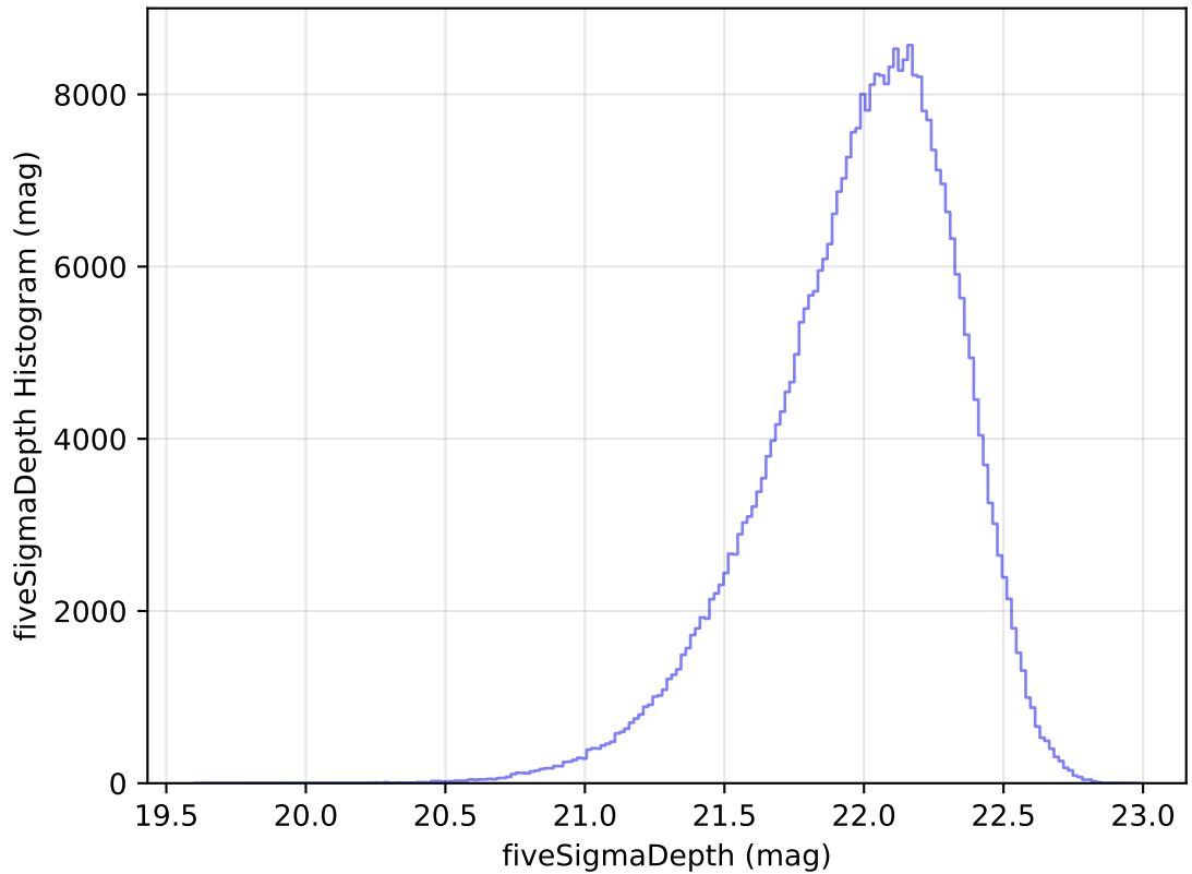
internal_u_expt27_nscale1.1v3.4_10yrs All sky y band: fiveSigmaDepth Histogram
