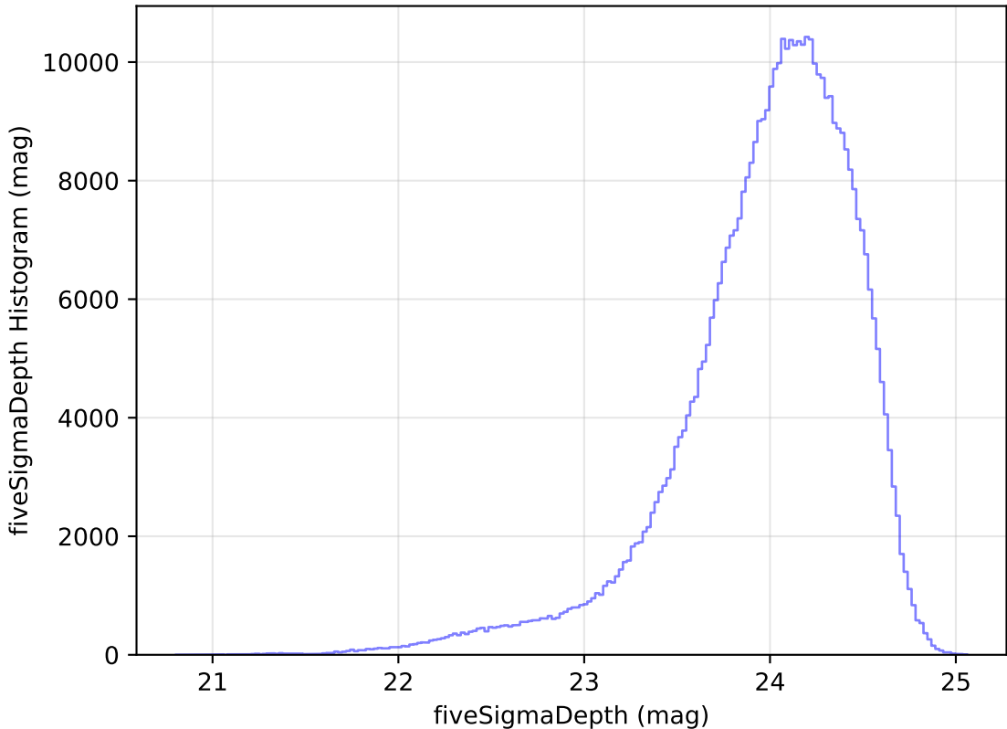
internal_u_expt27_nscale1.1v3.4_10yrs All sky r band: fiveSigmaDepth Histogram
