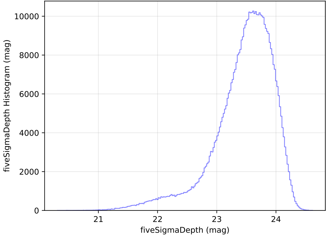
internal_u_expt27_nscale1.1v3.4_10yrs All sky i band: fiveSigmaDepth Histogram
