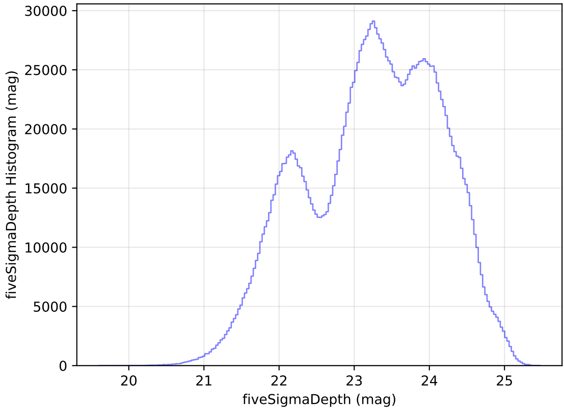
internal_u_expt27_nscale1.1v3.4_10yrs All sky all bands: fiveSigmaDepth Histogram
