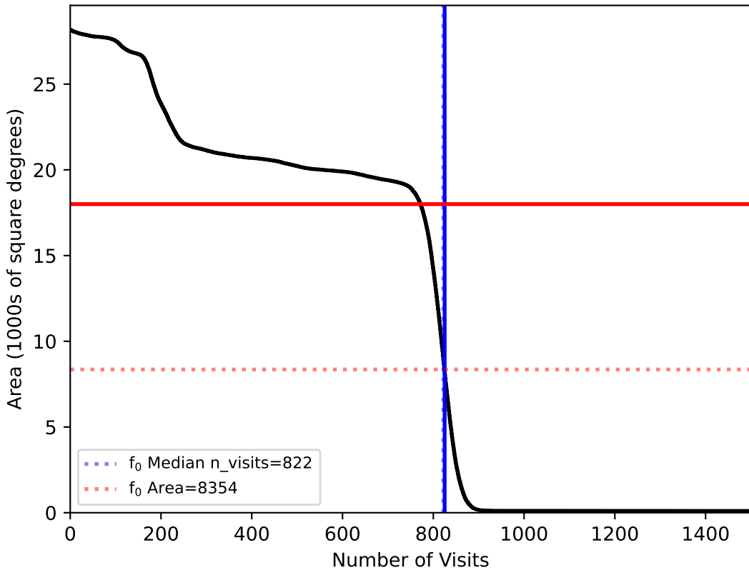
internal_u_expt27_nscale1.1v3.4_10yrs All sky: f0
