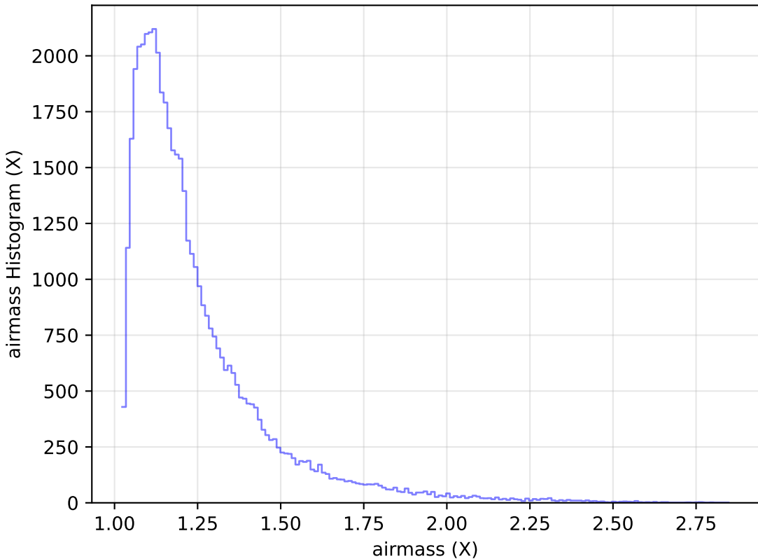
internal_u_expt27_nscale1.1v3.4_10yrs Yr 1 y band: airmass Histogram
