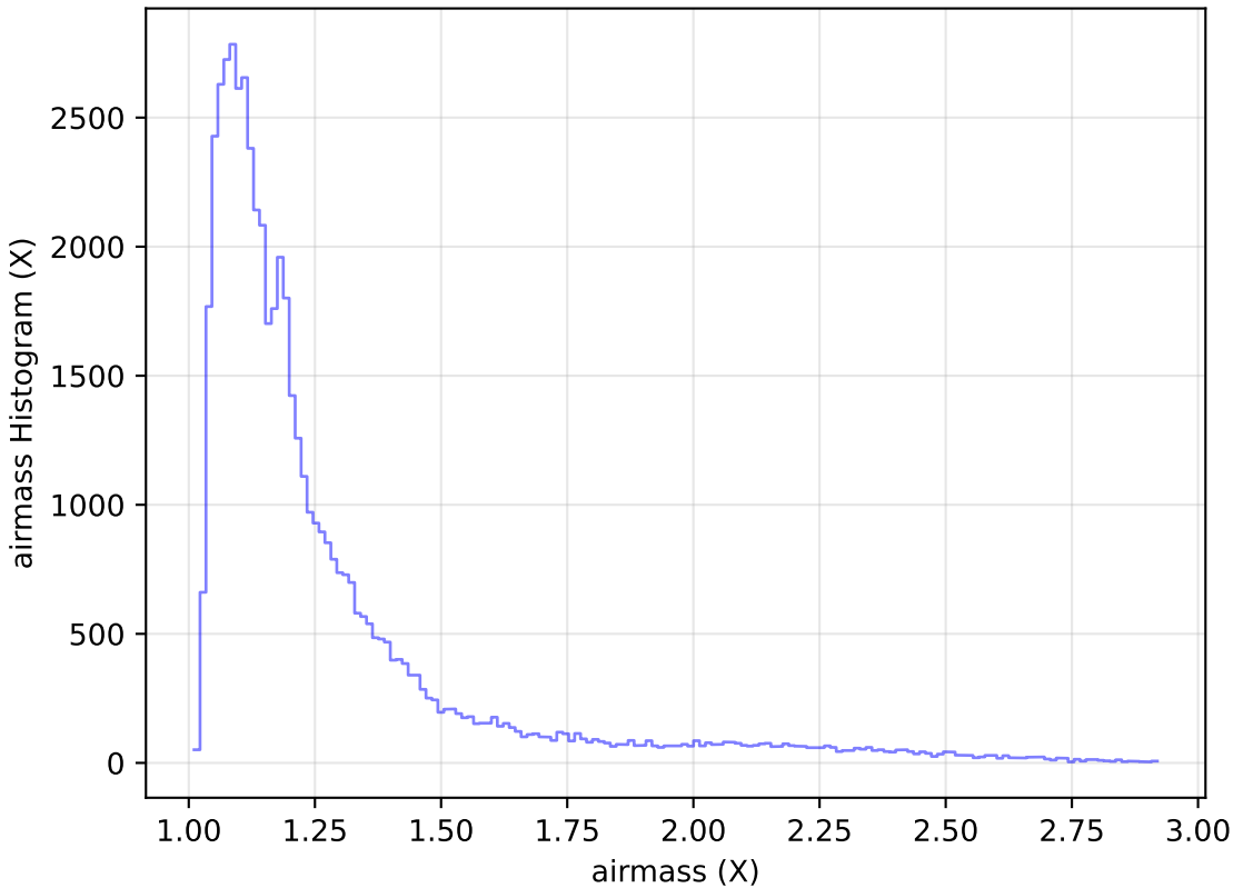
internal_u_expt27_nscale1.1v3.4_10yrs Yr 1 i band: airmass Histogram
