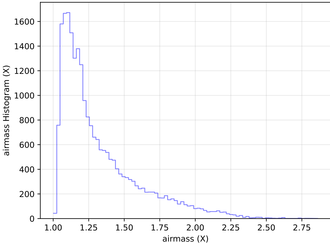
internal_u_expt27_nscale1.1v3.4_10yrs Yr 1 g band: airmass Histogram
