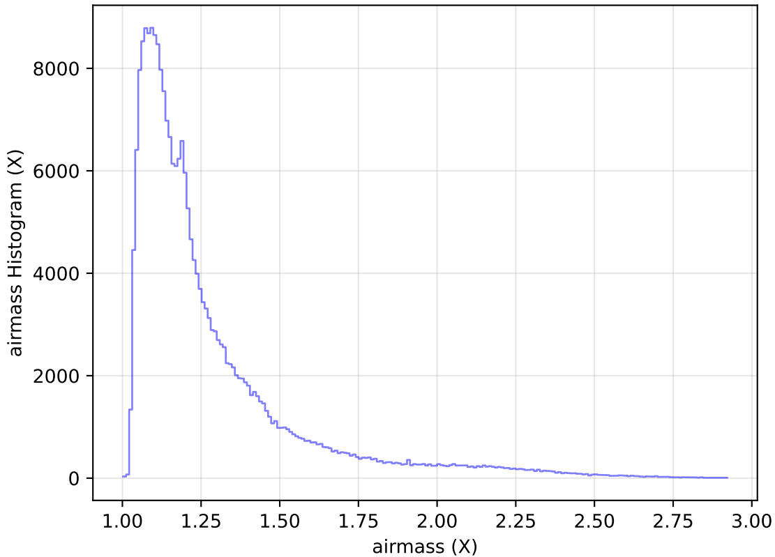
internal_u_expt27_nscale1.1v3.4_10yrs Yr 1 all bands: airmass Histogram
