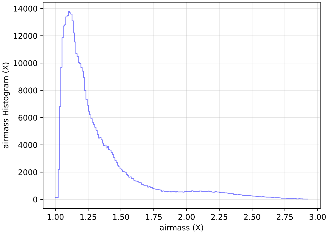
internal_u_expt27_nscale1.1v3.4_10yrs WFD z band: airmass Histogram
