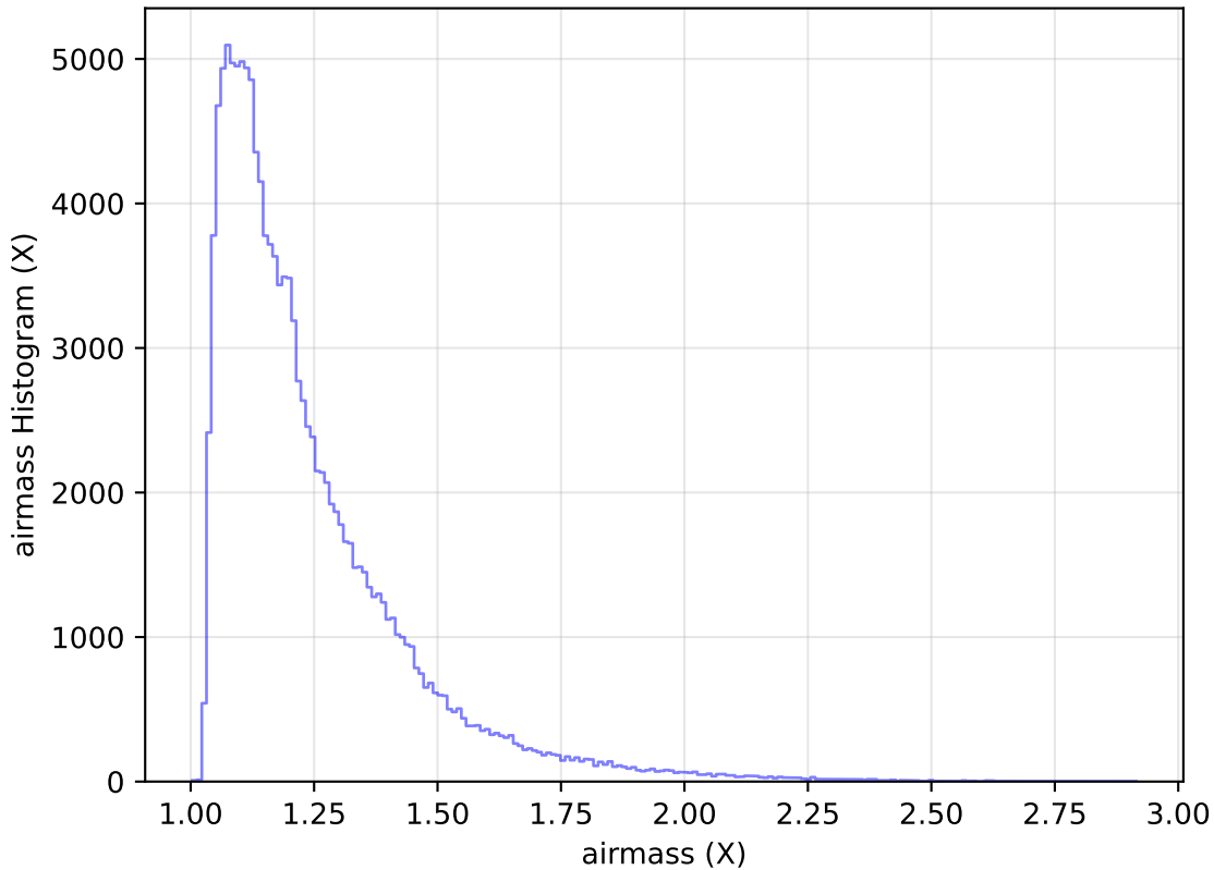
internal_u_expt27_nscale1.1v3.4_10yrs WFD u band: airmass Histogram
