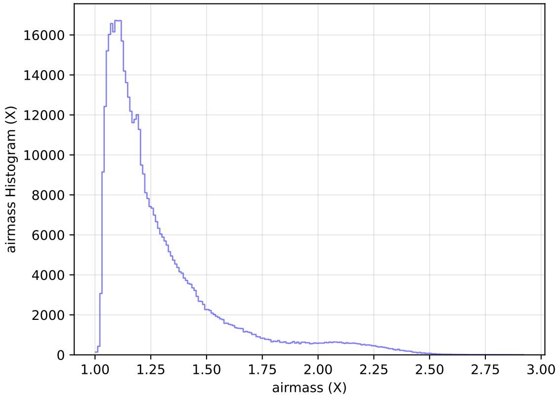
internal_u_expt27_nscale1.1v3.4_10yrs WFD r band: airmass Histogram
