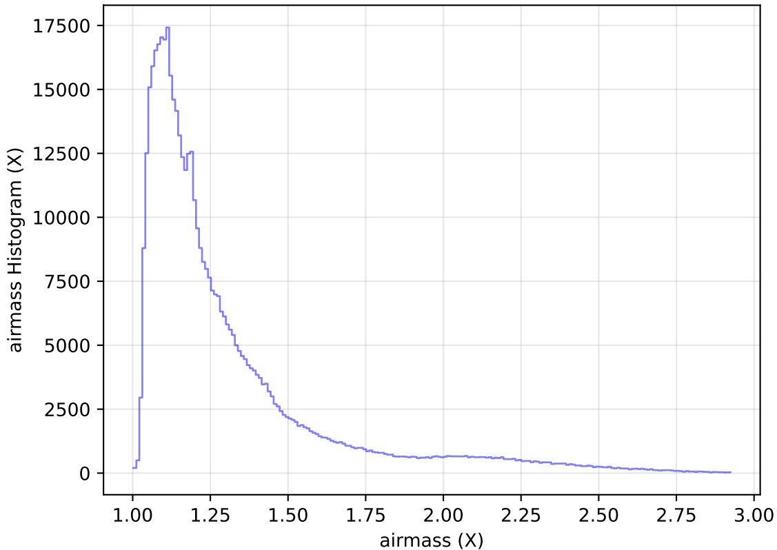
internal_u_expt27_nscale1.1v3.4_10yrs WFD i band: airmass Histogram
