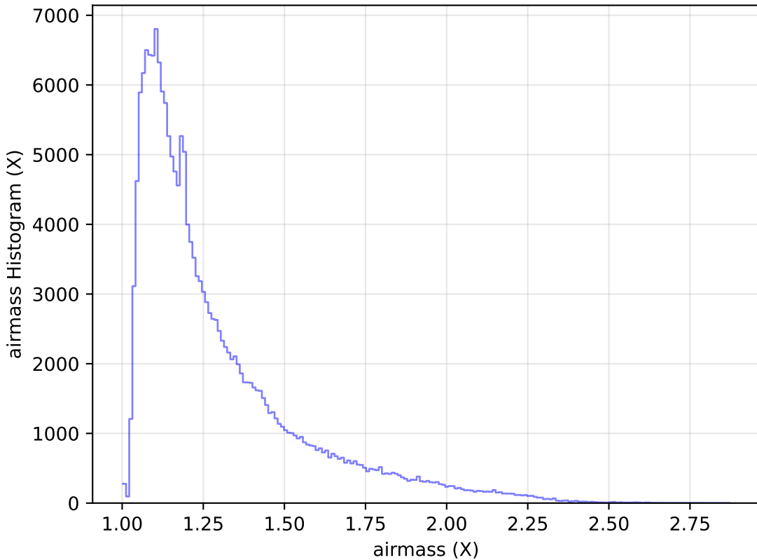
internal_u_expt27_nscale1.1v3.4_10yrs WFD g band: airmass Histogram
