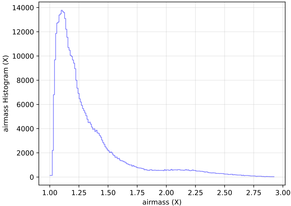
internal_u_expt27_nscale1.1v3.4_10yrs All sky z band: airmass Histogram
