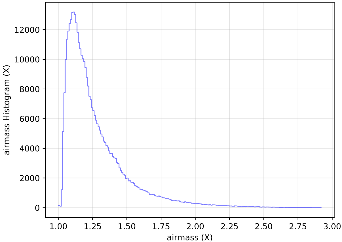
internal_u_expt27_nscale1.1v3.4_10yrs All sky y band: airmass Histogram
