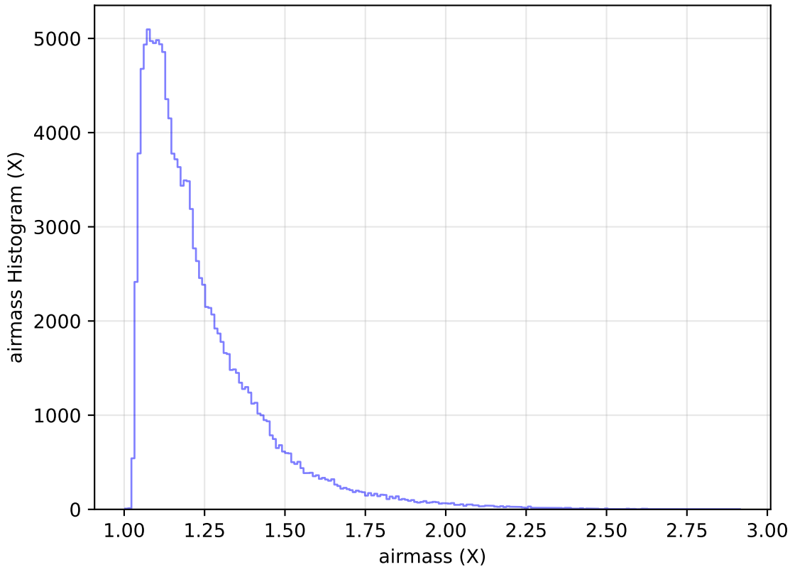
internal_u_expt27_nscale1.1v3.4_10yrs All sky u band: airmass Histogram
