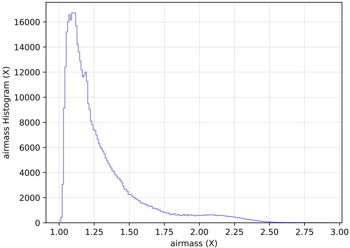
internal_u_expt27_nscale1.1v3.4_10yrs All sky r band: airmass Histogram
