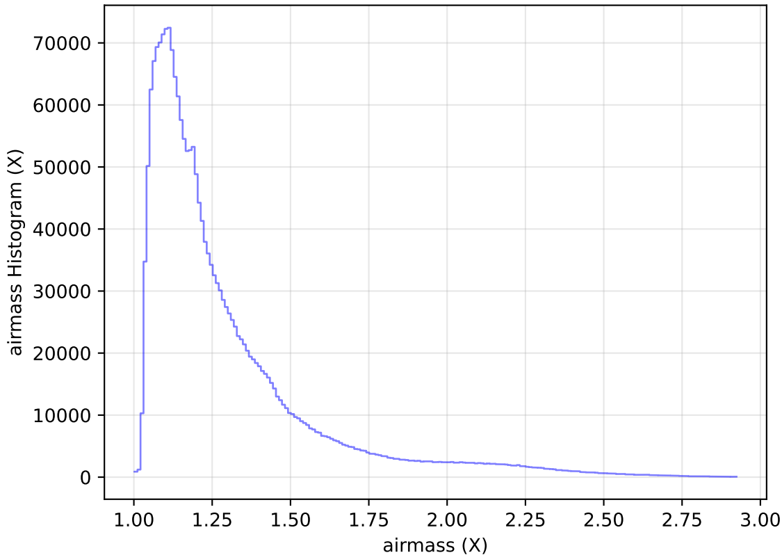
internal_u_expt27_nscale1.1v3.4_10yrs All sky all bands: airmass Histogram
