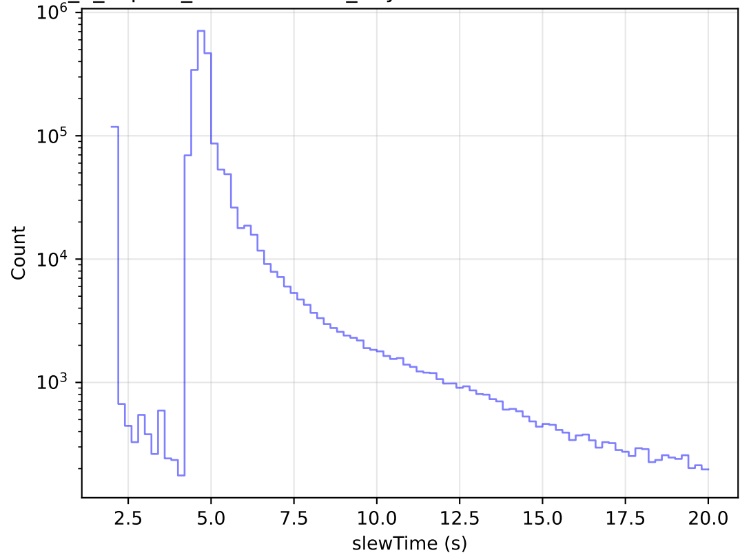
internal_u_expt27_nscale1.1v3.4_10yrs All visits: Zoom Slew Time Histogram
