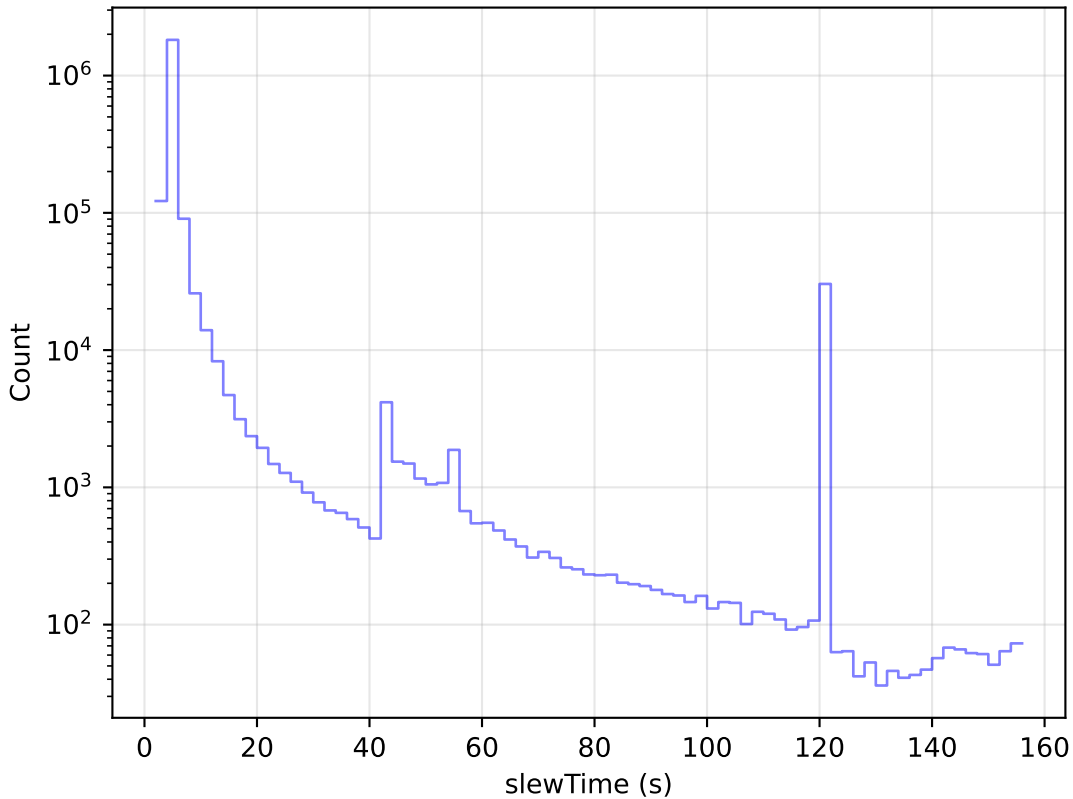
internal_u_expt27_nscale1.1v3.4_10yrs All visits: Slew Time Histogram
