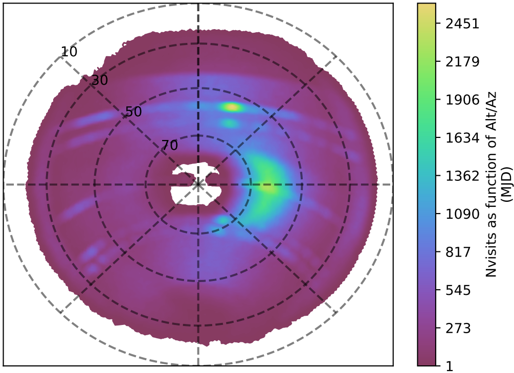
internal_u_expt27_nscale1.1v3.4_10yrs z band: Nvisits as function of Alt/Az
