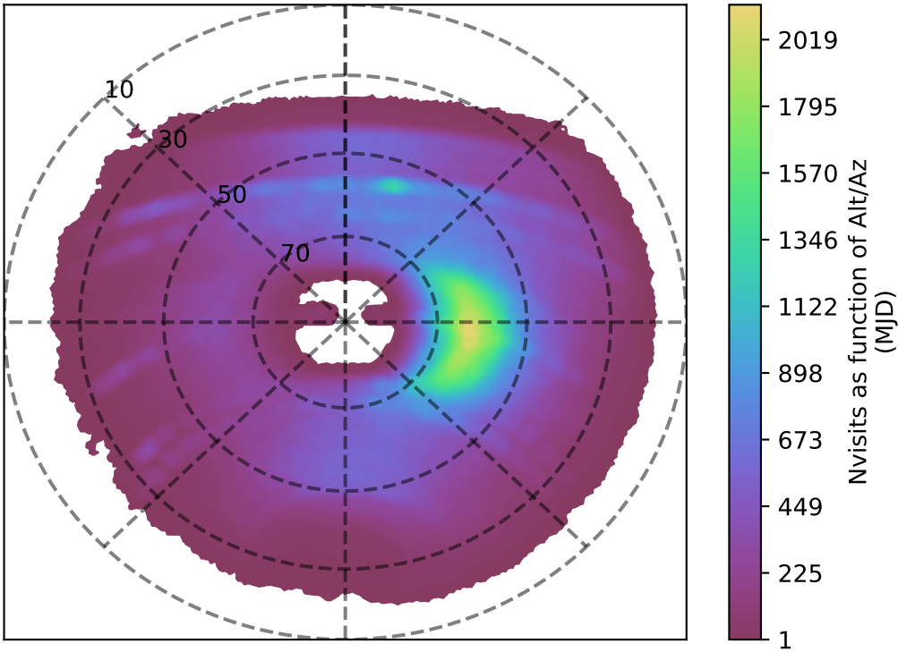
internal_u_expt27_nscale1.1v3.4_10yrs y band: Nvisits as function of Alt/Az
